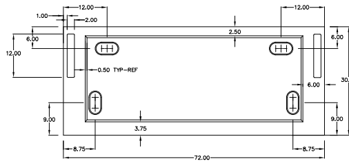
Work Surface (sold separately) - model numbers differ based on cupsink location
